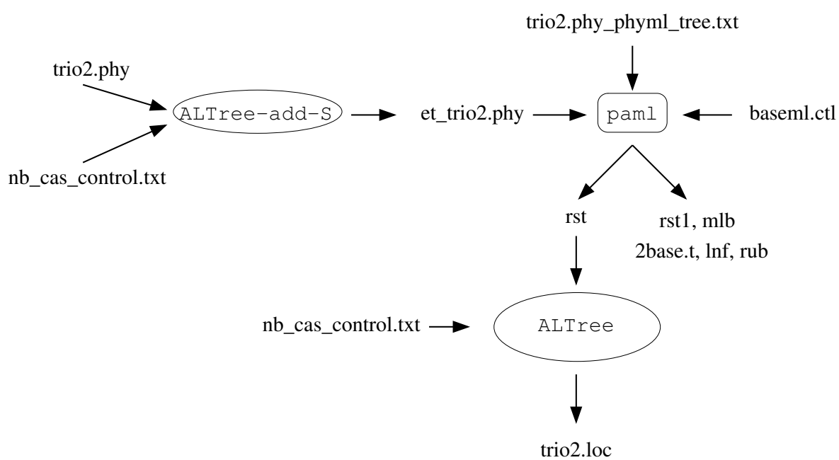
Figure VII: Summary of the different files and programs used for the localisation test (using pam1 )
