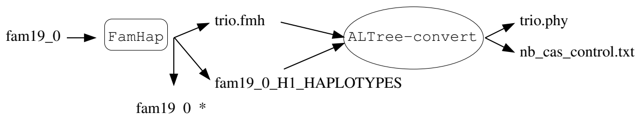
Figure II: Summary of the files and programs used to obtain input files for phylip or paml
