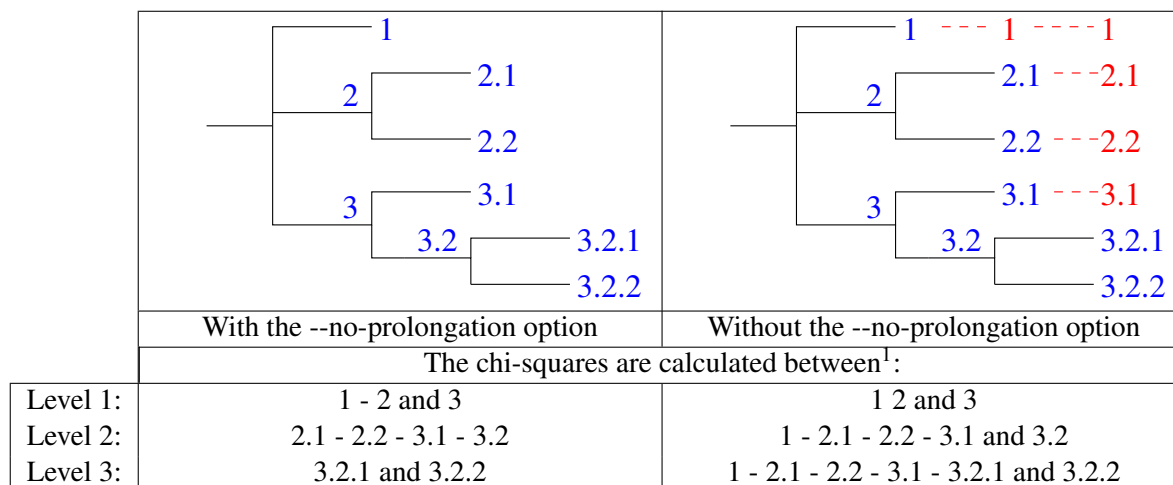
Figure I: Effect of the -b option
