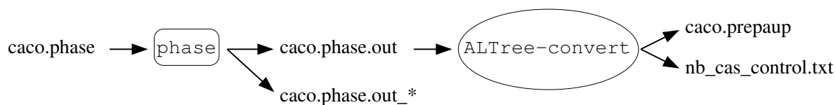
Figure I: Summary of the files and programs used to obtain input files for paup
