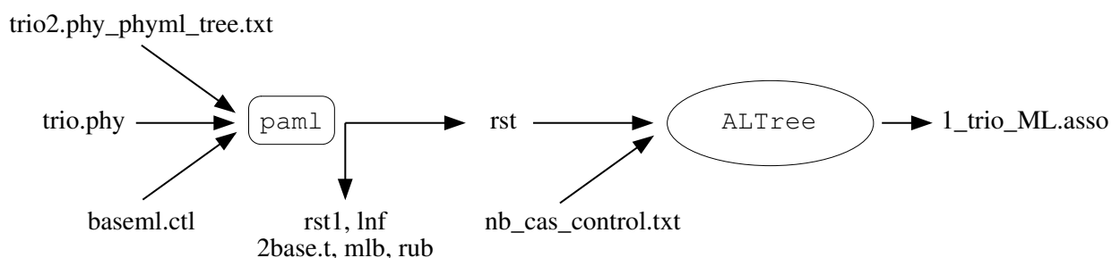
Figure VI: Summary of the different files and programs used for the association test (using pam1 )
