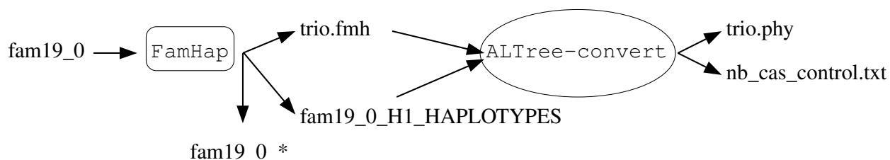
Figure II: Summary of the files and programs used to obtain input files for phylic or paml
